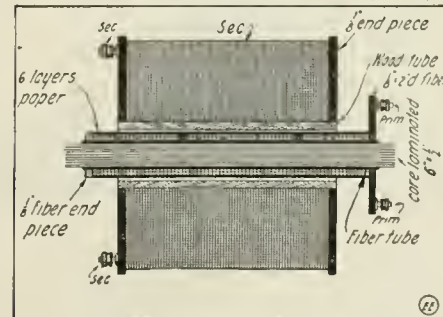
This Experimental Spark Coil Has a Removable Primary Coil and Core, So That All Sorts of Experiments Can Be Tried With It.
