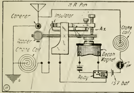
An Auxiliary Contact Fitted on the Relay of a Coherer Set Serves to Cut Off Local Oscillations from the Coherer.
