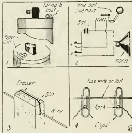
Some Handy Kinks for the Experimenter.
