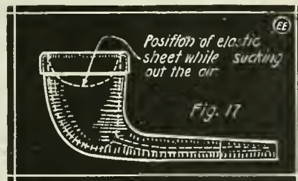
Removing the Air Within a Pipe Bowl by Sucking In Thru Stem Allows the Pressure of the Air to Push Elastic Diaphragm Inward.
