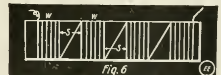
Radio Inductances Have Their Distributed Capacity Reduced by Winding the Coils in Groups, With a Space Between.
