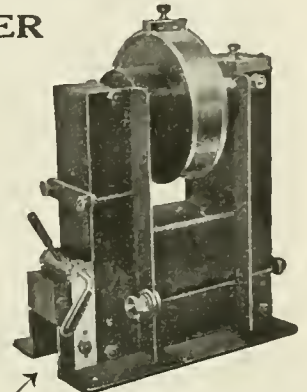
The Variable Shunt (marked by arrow) is an exclusive Thordarson feature enabling the operator to obtain perfect resonance by regulating the air-gap. Locked in position by eccentric cam.
