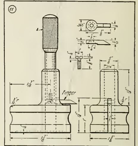
An Effective Precision Height Gage May Be Constructed from a Standard Micrometer Head Fitted in a Steel Base of the Dimensions Indicated.
