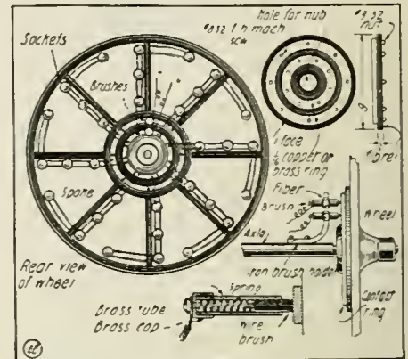
Details of Sulky Wheels and the Metal Contact Rings and Brushes Whereby Current is Conducted to the Lights on the Spokes.
