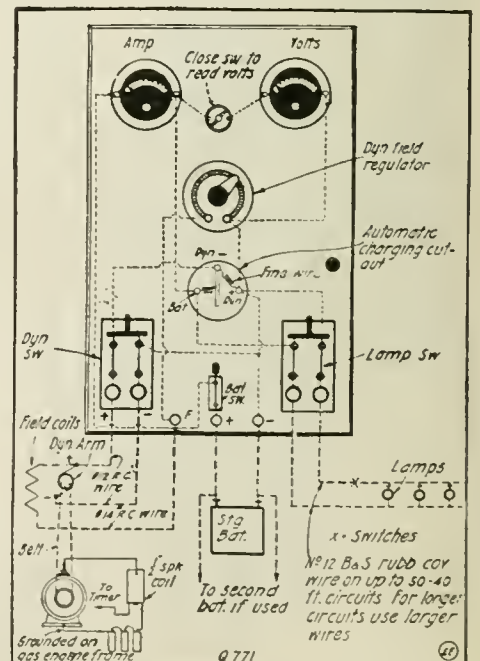
Wiring Diagram for 32 Volt Lighting Plant.
