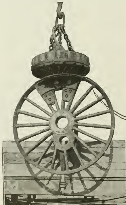
43-inch Magnet Lifting a Locomotive Drive Wheel at the West Milwaukee Shop of the C. M. & St. Paul Railway. Another Instance of What the Lifting Magnet Is Capable of Doing.
