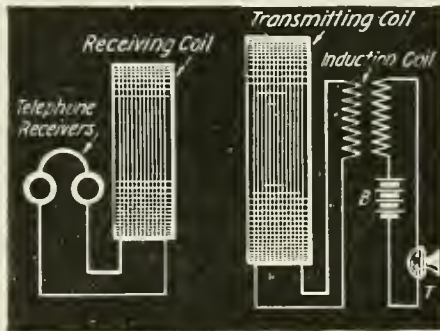
Hook-up for Inductive Wireless 'Phone.
