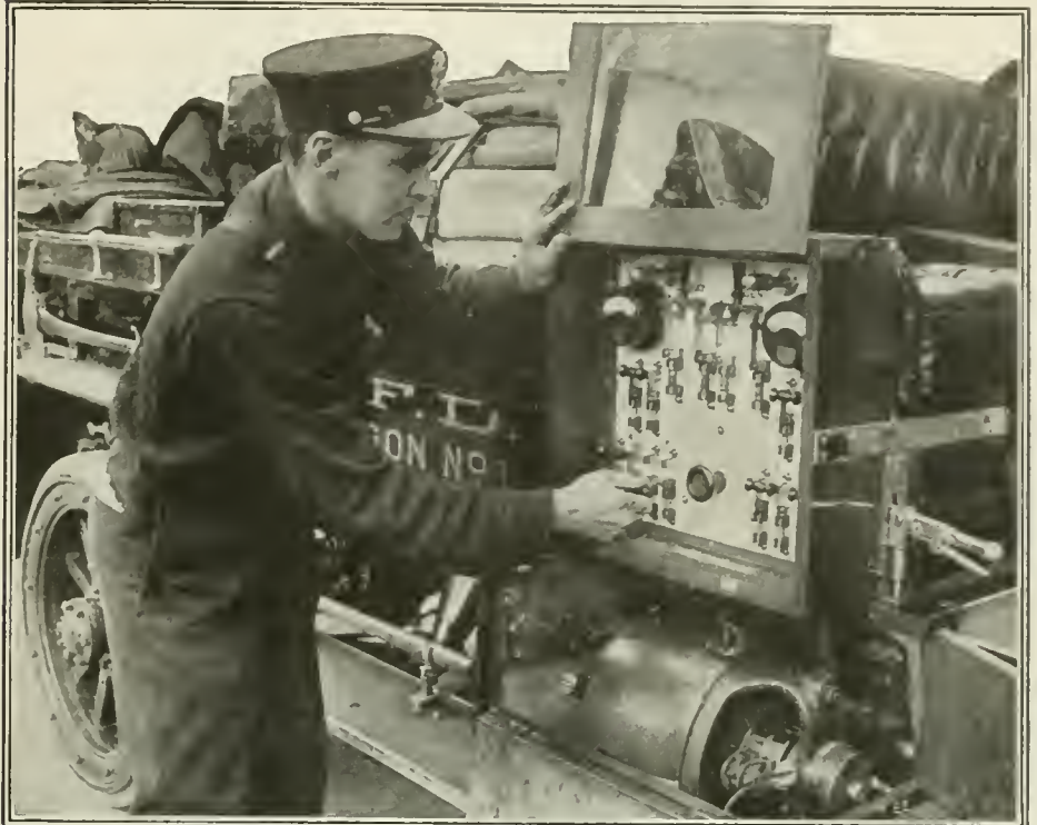
Los Angeles, Cal., Boasts of Having One of the Most Complete Electric Fire-fighting Trucks in the United States. The Equipment Comprises Five Powerful Searchlights Which are Supplied with Power from Either a Large Storage Battery or the Dynamo Shown in the Picture.
