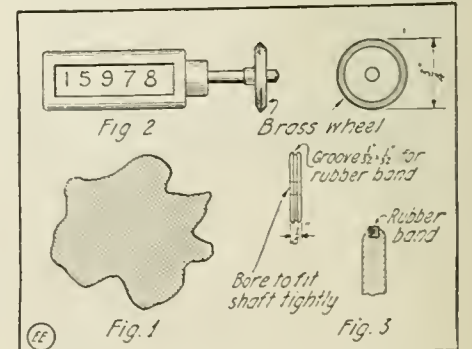
Attachment for a Speed Indicator Making It Available for Measuring the Perimeter of Irregular Surfaces, Map Routes, etc.
