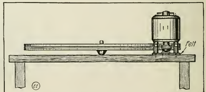
Where It is Not Possible to Conceal the Motor in the Cabinet, as in Small Machines, the Motor Can Be Readily Mounted Above the Cabinet Shelf as Shown. (Fig. 2.)
