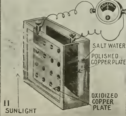
PHOTO-ELECTRIC CELL
