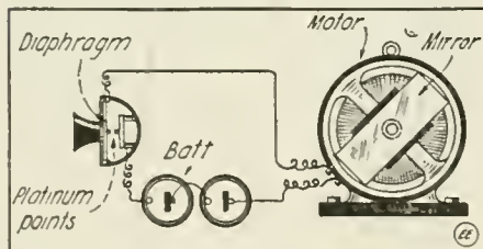
Novel Scheme for Controlling Revolving Mirror by Means of a Microphone.
