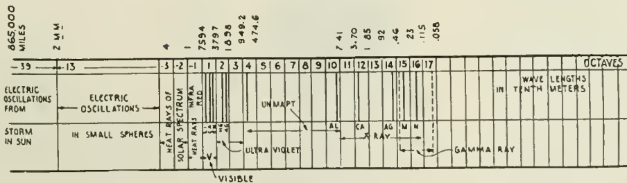
Fig. 2. Chart Showing the Position Occupied by the New "R-Ray" in the Spectrum, Including the Relative Position of the X-Ray Vibrations and Ultra-Violet Rays.
