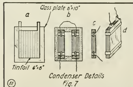
Details for Building High Tension Glass Plate Condenser to Be Connected in Tesla Coil Circuit.
