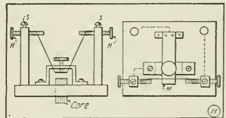
We All Desire to Have a High Note Spark. Here's How—A Piece of German Silver Wire Serves to Hold Back the Free End of the Vibrator Spring, Reducing Its Swing and Raising the Frequency.
